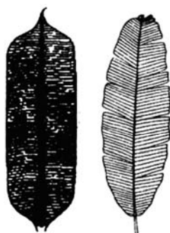
Parallel pinnate (Unicostate)
